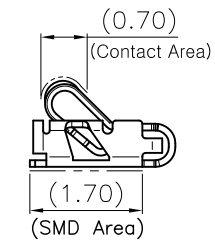
PLATING AREA
