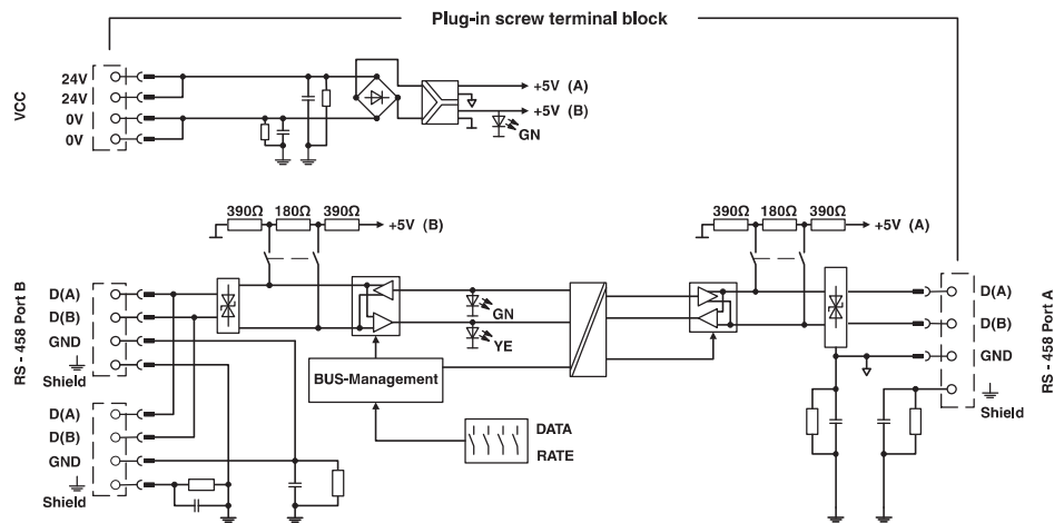
Circuit diagram
